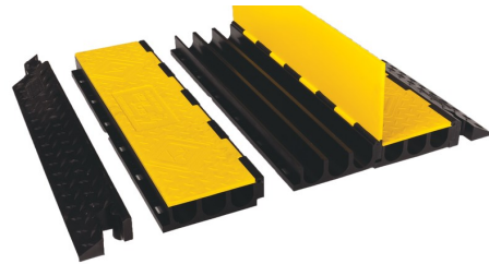
Modular Cable Protector Systems Up to 35,600lbs/Axle Capacity
